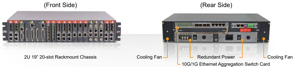
10G/1G Ethernet Aggregation Switch Card
