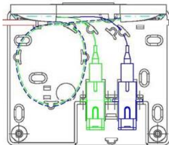
MCPE-02-SC A/SC S-A two SC pigtails
