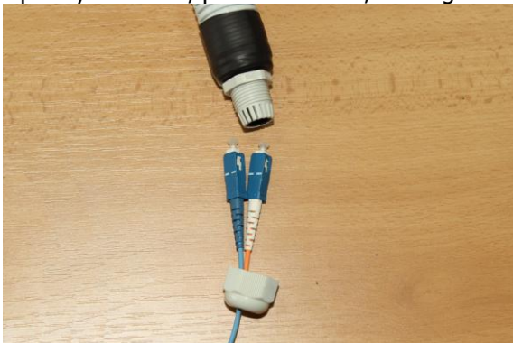
Nut of cable gland is moved over connectors
