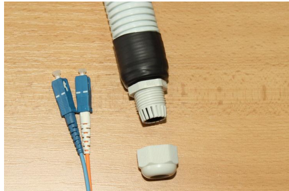
Duplex cable to be inserted into protection tube
